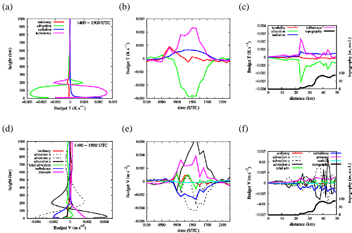
Figure 2.4. Temperature and wind speed budgets in the Campos basin (see location in the red point in Fig. 2.1). (a) and (d) Vertical profiles of the averaged budgets (from 1400 to 1500 UTC, mature phase). (b) and (e) Time series of the budgets at 10 m (a.g.l.). (c) and (f) Spatial evolution of the averaged terms (1400-1500 UTC) along the green line in Fig 2.1, together with the topography.
