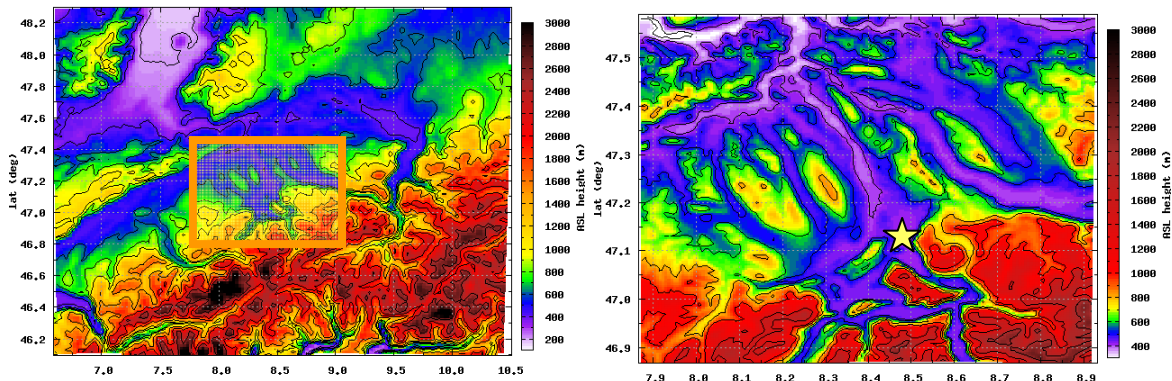
Figure 4.1. Topography of the inner and outer domains. The star indicated the location of Chamau, the main measurement site of the campaign.
