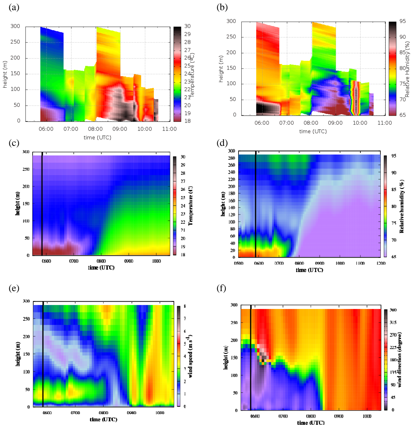
Figure 2.5. Balloon soundings during 20 th September 2013 (IOP of MSB13 experimental field) for (a) temperature and (b) relative humidity. The same in (c) and (d) but for the model outputs. The wind speed (e) and direction (f) obtained from the model outputs in this site is also included.
