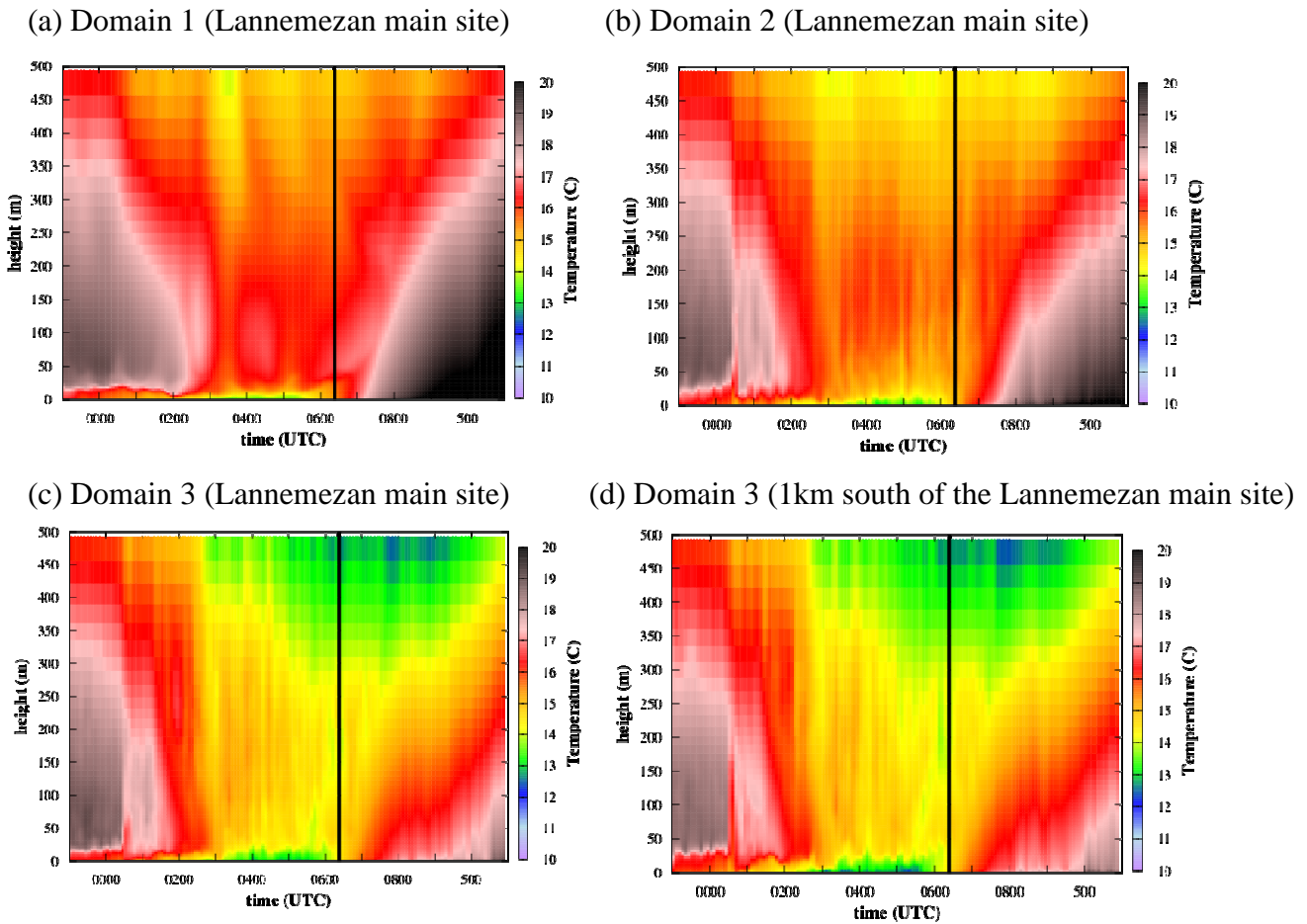
Figure 1.5. The same as Figure 1.4 but for the temperature.
