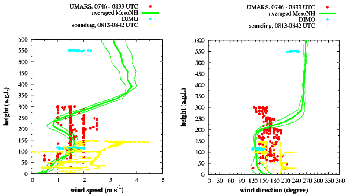
Figure 4.4. Comparison of the model results (in green) to the available observations. Data from the flights in red (small UAV) and in blue (piloted aircraft) and profiles from the sounding in yellow. The model outputs are averaged over the period of the UMARS flight and in this plot is shown the mean value (thick green line) and the standard deviation (thin green line).
