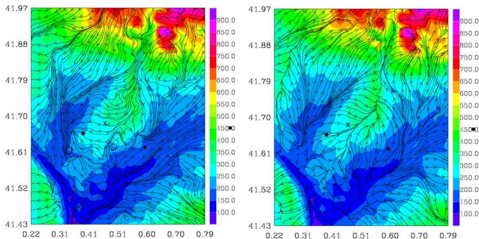
Figure 3.7. Streamlines at 15m (a.g.l.) obtained from the outer domain but for a zoom in the area of interest. The location of Raimat, where the experimental field campaign was done, is indicated with a cross.
