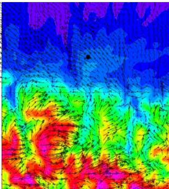
Figure 1.2. Wind vectors at 50 m (a.g.l.) at 2330 UTC on July 1 st , 2011 for (a) 2km resolution domain ( D1 ) with a zoom over the domain 2 area and (b) 400m resolution domain ( D2 ).
