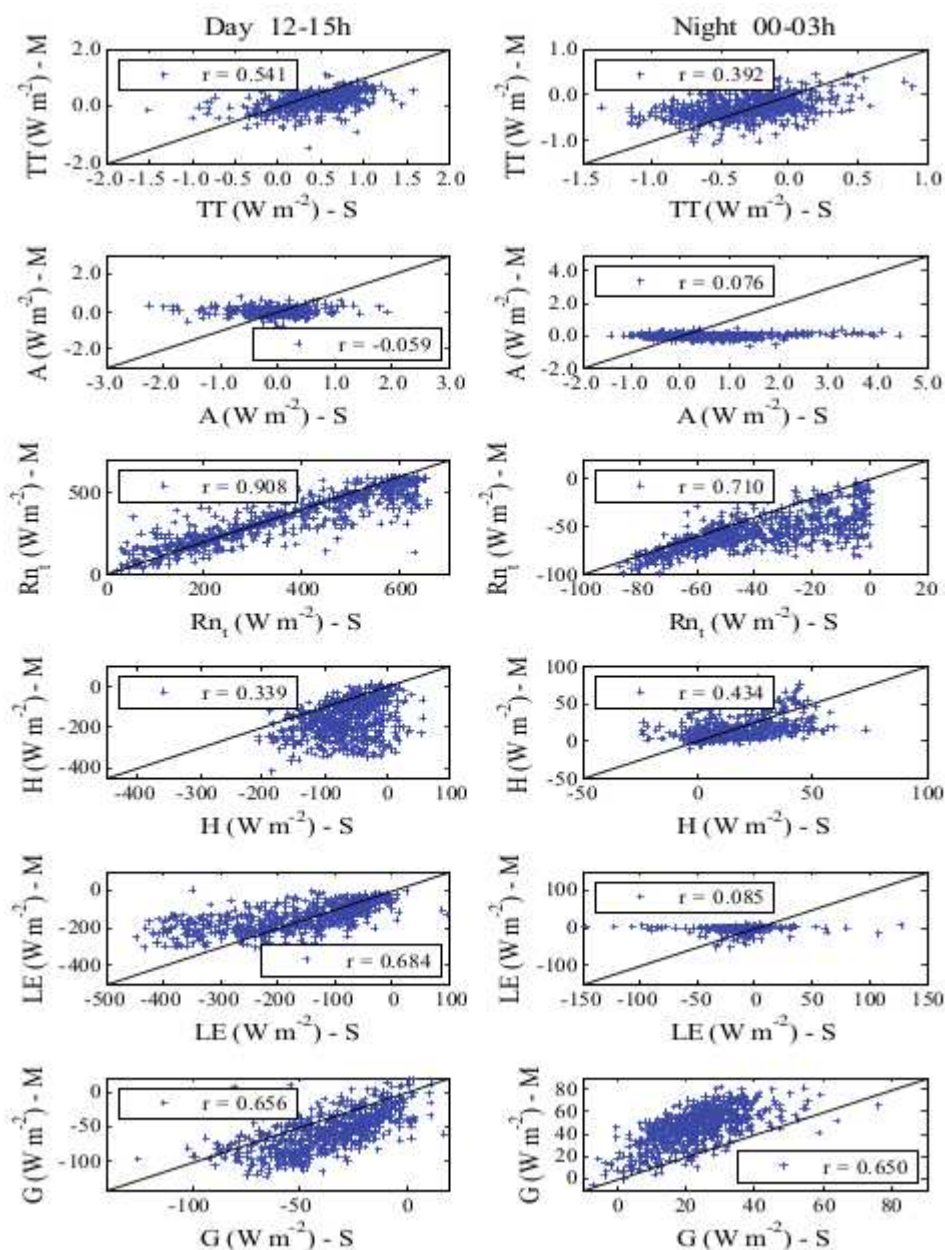
Fig. 5.3. Correlation between the observed values (labelled with S) with those simulated (M) for all the data during 2009 and 2010.
