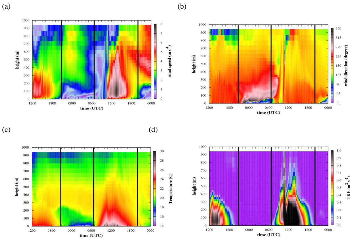
Figure 2.3. Time series of the vertical profiles obtained from the model in the location indicated with a red dot in Fig. 2.1 (where the experimental field campaigns will be performed).
