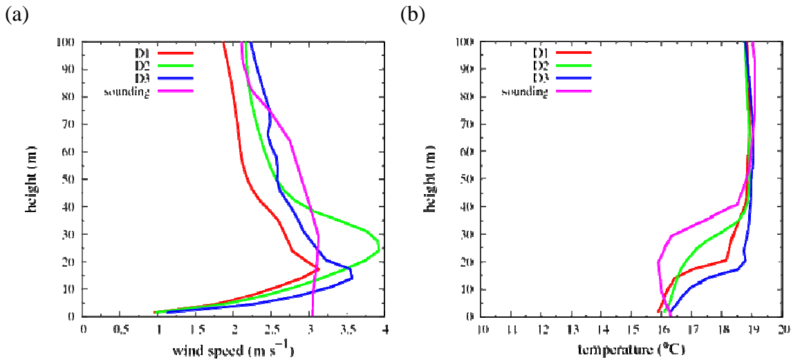
Figure 1.6. Vertical profiles obtained by the 3 model domains in Lannemezan at 2330 UTC. The observed sounding at the same time (in purple) is included.
