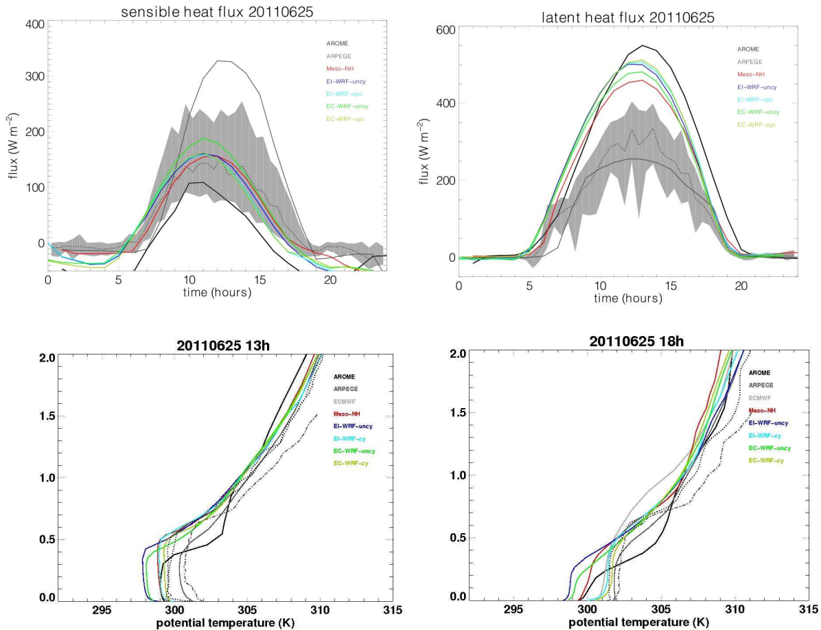
Figure 1.7. Time series for (a) H and (b) LE observed (mean value and standard deviation in grey) and obtained from the different models that participate in the intercomparison. Vertical profiles of the potential temperature at (c) 1300 UTC and (d) 1800 UTC. The observed soundings are also included (dashed lines).
