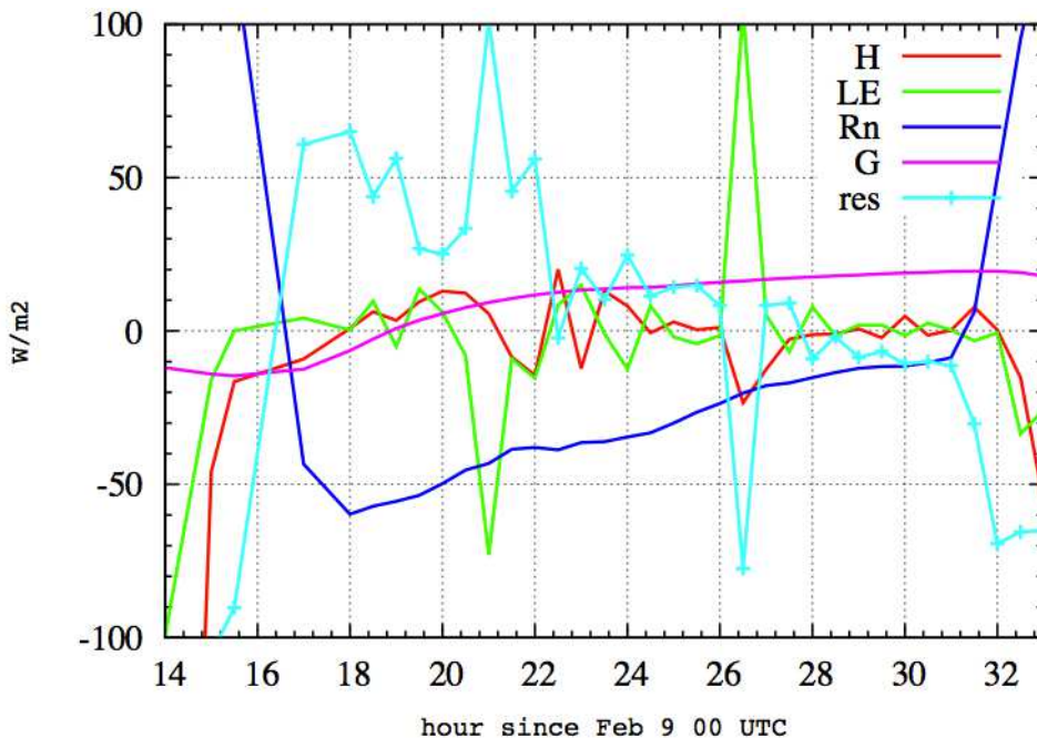
Figure 3.2. Observed surface energy balance in Raimat centered in the night 9-10 February.
