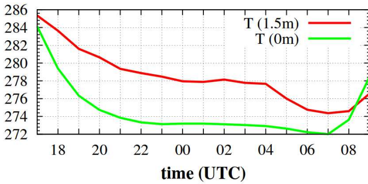
Figure 3.8. (a) and (b) Time series of the vertical profiles of the wind speed and direction, respectively. (c) Temporal evolution of the modelled temperature at 1.5m and at the ground for Raimat during night 9-10 February 2011.
