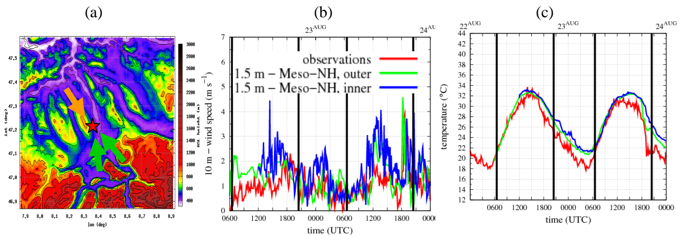
Figure 4.2. (a) Wind direction during the day (orange arrow) and during the night (green arrow) in Chamau (red star) obtained from the model outputs. (b) and (c) Comparison of the model results to the observations in Chamau.
