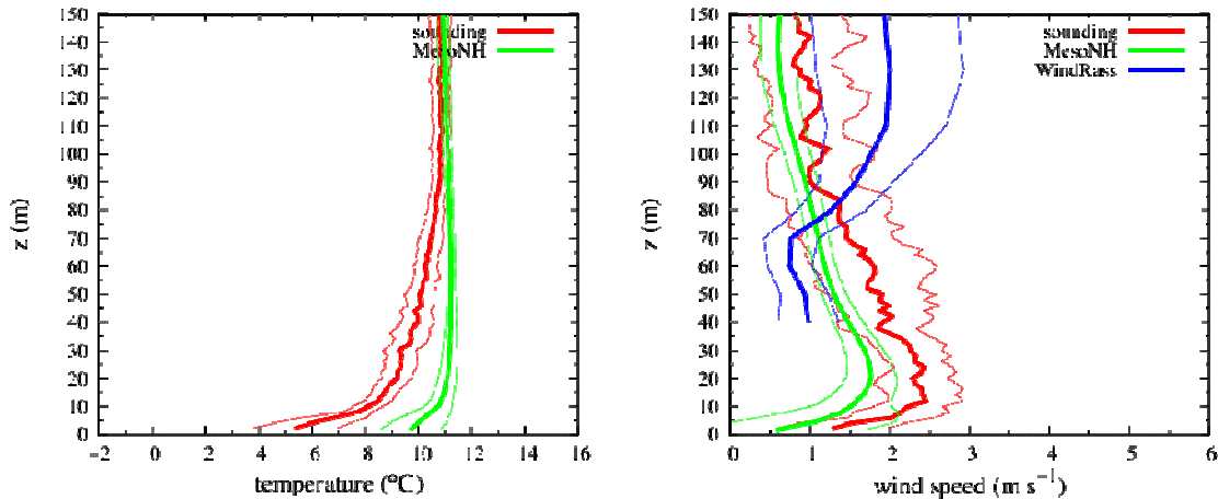
Figure 3.1. Averaged soundings during the evening together with the same data from the simulation.
