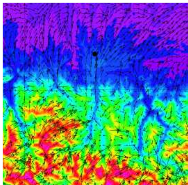
Figure 1.2. Wind vectors at 50 m (a.g.l.) at 2330 UTC on July 1 st , 2011 for (a) 2km resolution domain ( D1 ) with a zoom over the domain 2 area and (b) 400m resolution domain ( D2 ).
