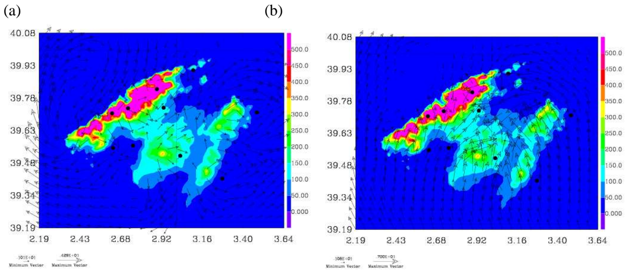
Figure 2.2. Wind vectors at 10m (a.g.l.) at (a) 0500 UTC on 5 th June 2010 and at (b) 1200 UTC.
