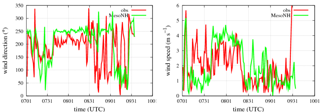
Figure 4.3. (a) Flight path of the measurement flights made by DIMO HB-2335, operated by MetAir AG during the experimental field campaign together with the topography of the area. (b) and (c) wind speed and direction observed (red line) during the evening and next morning, respectively, together with the model results (green line).
