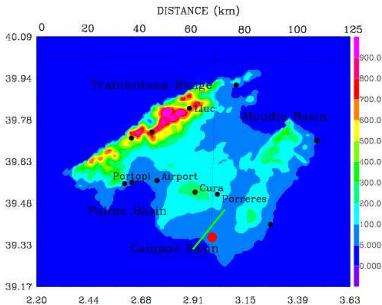
Figure 2.1. Topography of the Island of Majorca. This area corresponds to the inner domain (at 1km resolution) of the run.
