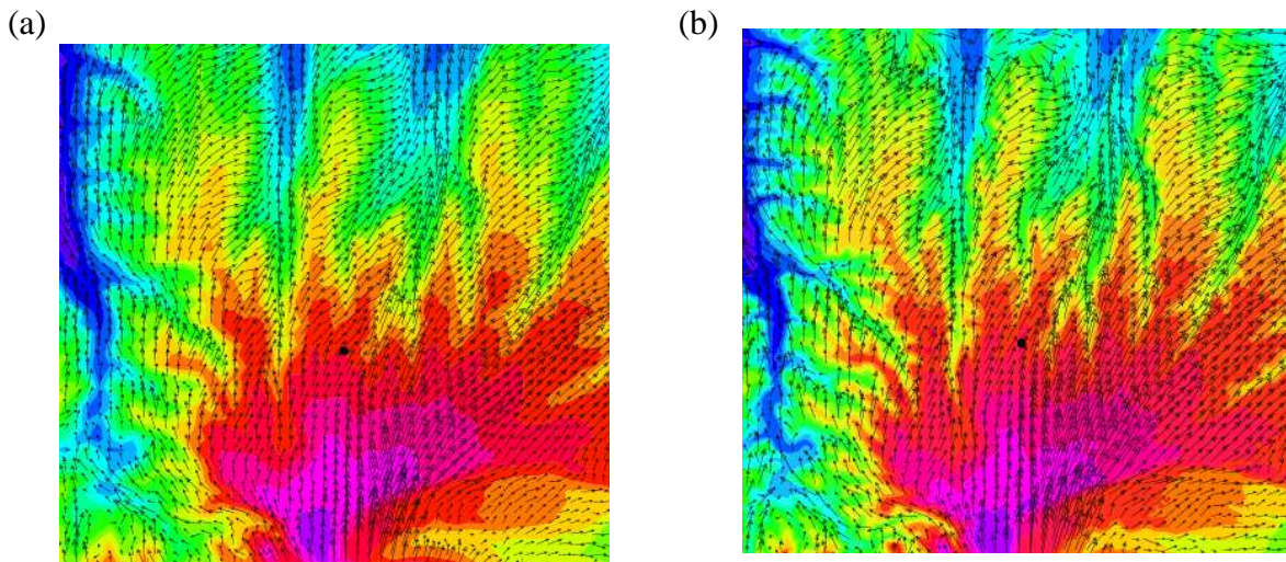
Figure 1.3. Wind vectors at 50 m (a.g.l.) at 2330 UTC on July 1 st , 2011 for (a) 400m resolution domain (D2) with a zoom over the domain 3 area and (b) 80m resolution domain (D3).
