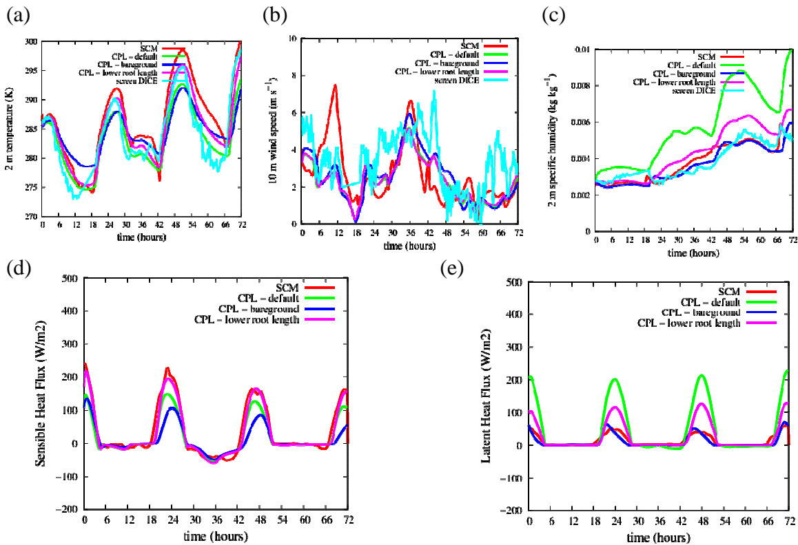
Fig. 5.2. DICE results obtained from the MesoNH model: stage 1 (SCM) and stage 2 (CPL, several sensitivity tests). In light blue the observations. Time series of: (a) 2m temperature, (b) 10m wind, (c) 2m specific humidity, (d) sensible heat flux and (e) latent heat flux.
