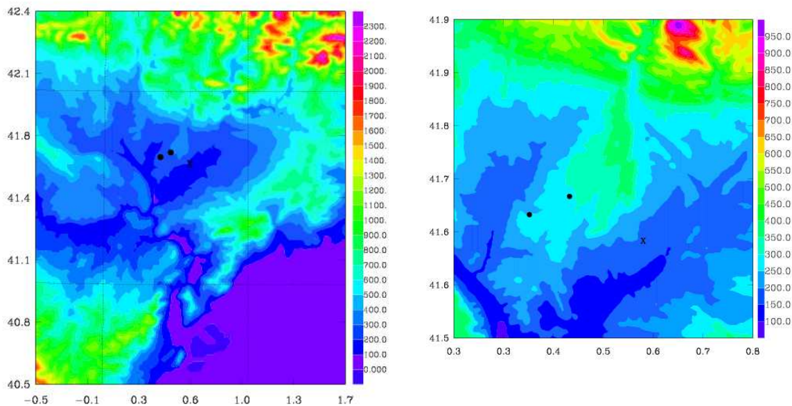
Figure 3.6. Inner and outer domains of the strong nocturnal inversion case in Raimat.
